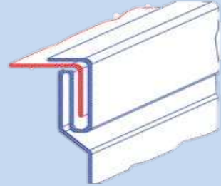
Pittsburgh Lock
