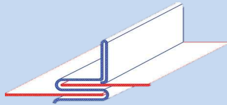
Standing "S" Cleat (SMACNA - T11)
