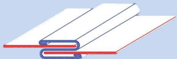
Hemmed "S" Cleat (SMACNA - T6)
