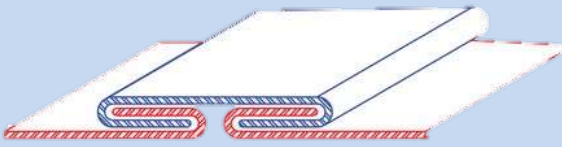
Drive Cleat (SMACNA - T1)
