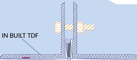
Companion Angles
